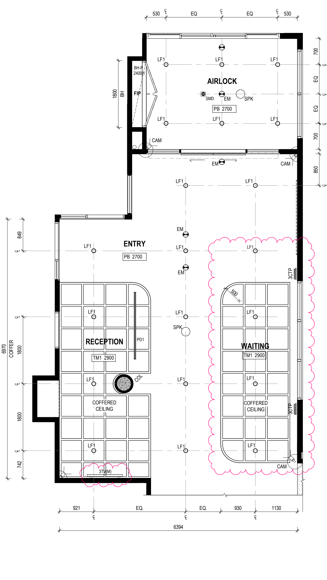
2 RCP - VILLAGE ARRIVALS - AIRLOCK, RECEPTION, LOBBY & WAITING Scale 1: 50
