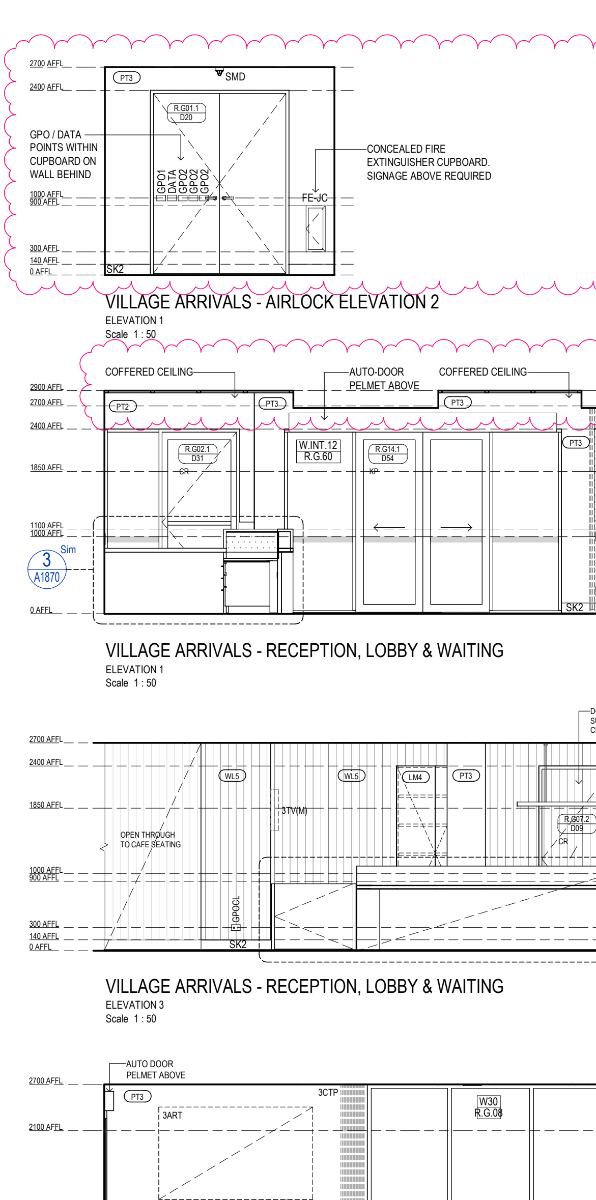
VILLAGE ARRIVALS - RECEPTION, LOBBY & WAITING Scale 1: 50
